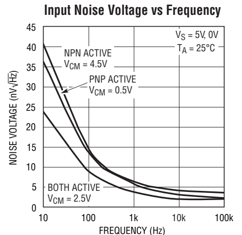
LT6202/03/04 G18
