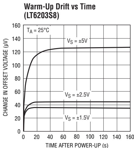
LT6202/03/04 G16
