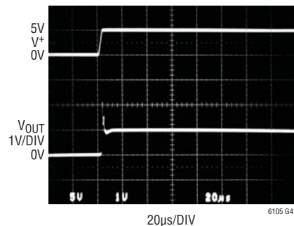
Power Supply Start-Up Response
