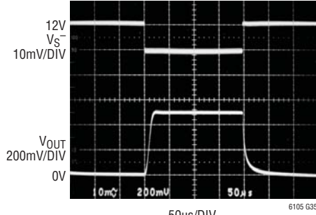
Step Response V_{SENSE} = 0V \text{ to } 10mV, V_S^+ = 12V
