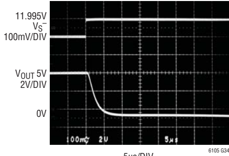
Step Response V_{SENSE} = 100mV \text{ to } 5mV
