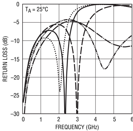
Return Loss vs Frequency Reference in Figure 1 Test Circuit
