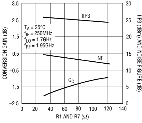
Figure 6. IIP3, G C and Noise Figure vs External Resistance, Constant Core Current (Variable Supply Voltage)
