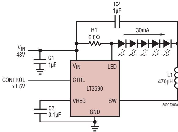
48V Supply for 5 LED String, 30mA Current
