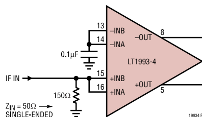
Figure 1. Input Termination for Single-Ended 50Ω Input Impedance
