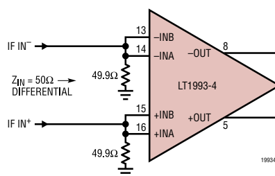
Figure 2. Input Termination for Differential 50Ω Input Impedance
