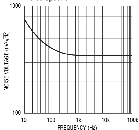
LT1460S3-2.5V Output Voltage Noise Spectrum
