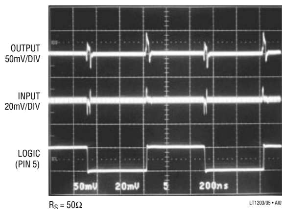
LT1203 Channel-to-Channel Switching Transient
