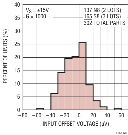
Distribution of Input Offset Voltage, TA = -40°C
