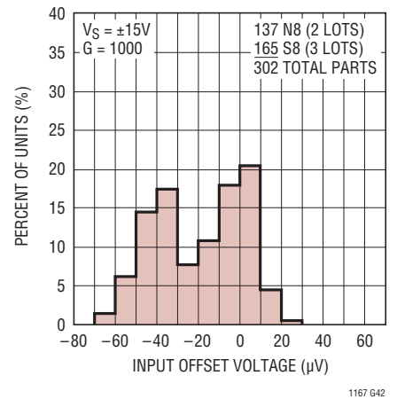
Distribution of Input Offset Voltage, TA = 85°C
