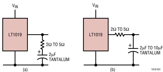
Figure 1. Output Bypassing
