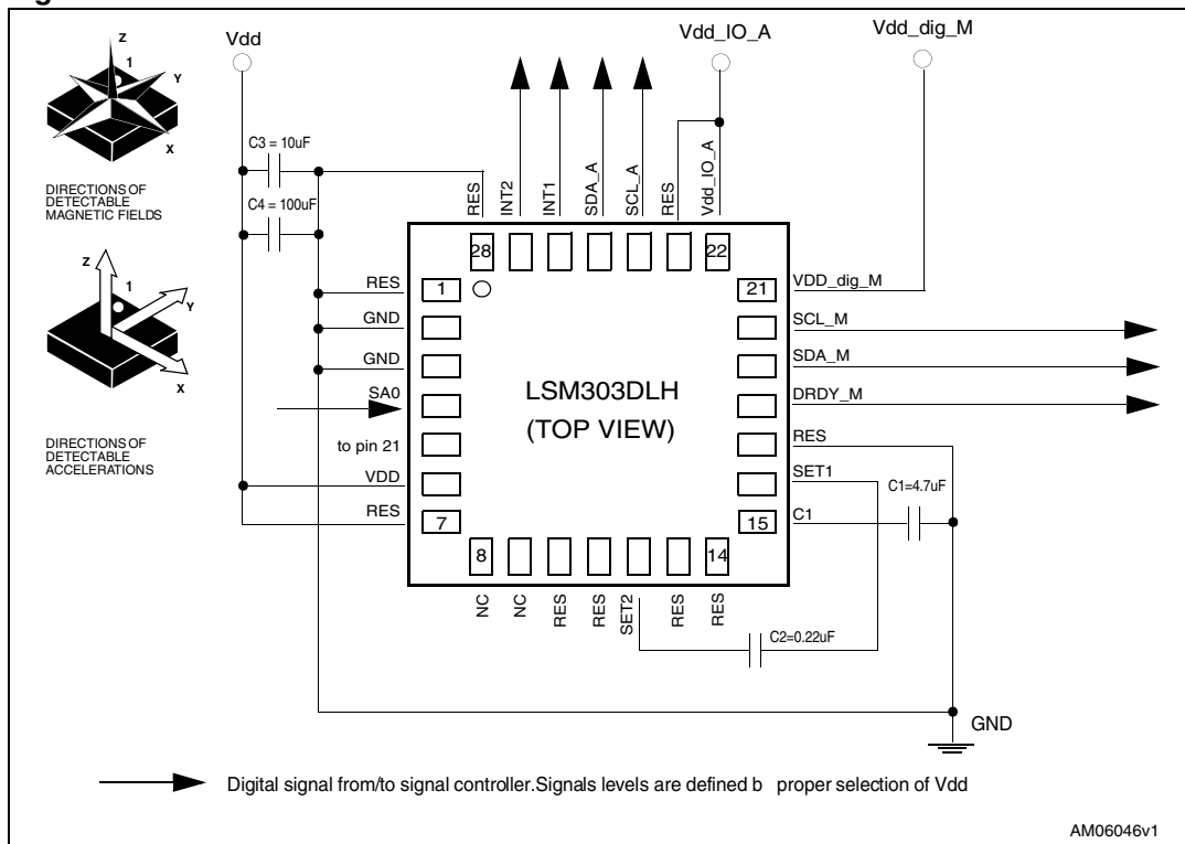
Figure 5. LSM303DLH electrical connection 2
