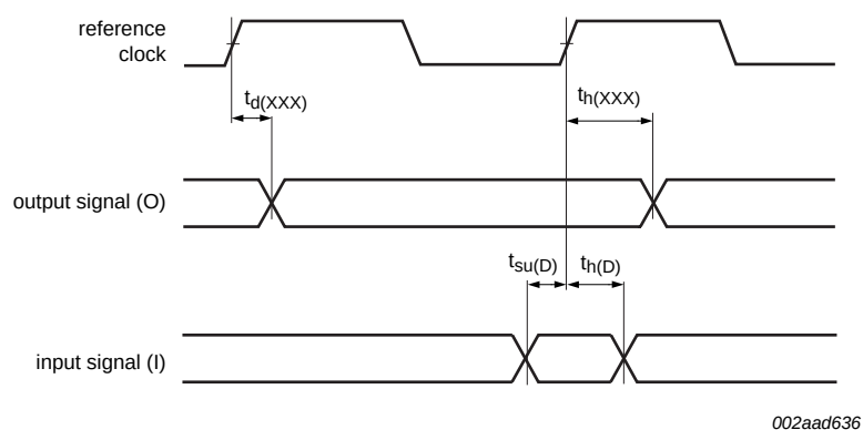
Fig 17. Signal timing
