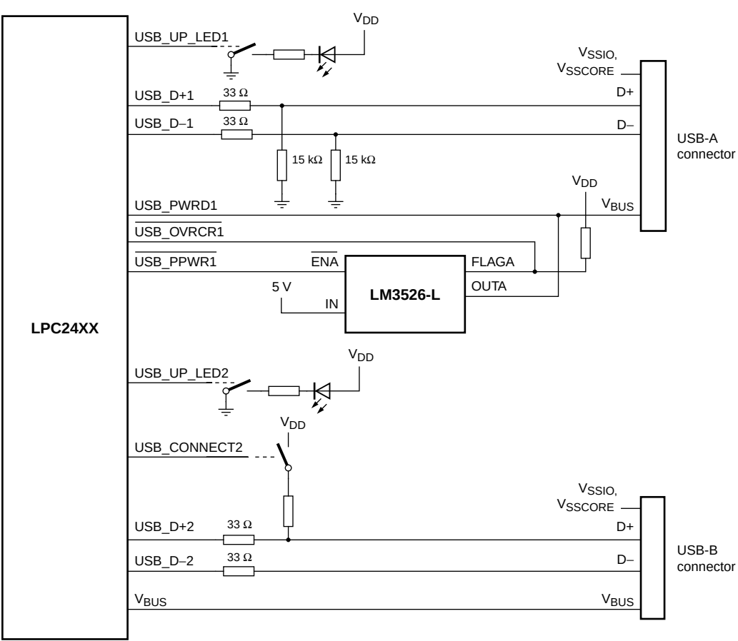
Fig 24. LPC2458 USB OTG port configuration: USB port 2 device, USB port 1 host
