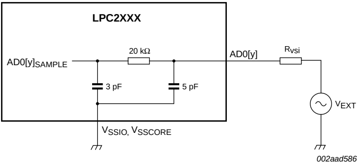
Fig 19. Suggested ADC interface - LPC2458 AD0[y] pin
