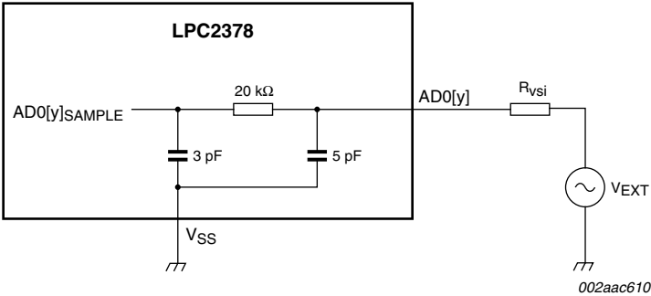
Fig 5. Suggested ADC interface - LPC2388 AD0[y] pin
