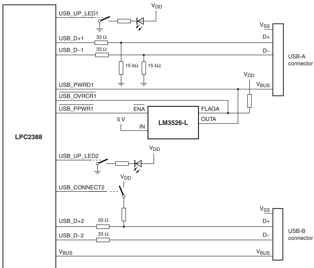
Fig 13. LPC2388 USB OTG port configuration: USB port 2 device, USB port 1 host
