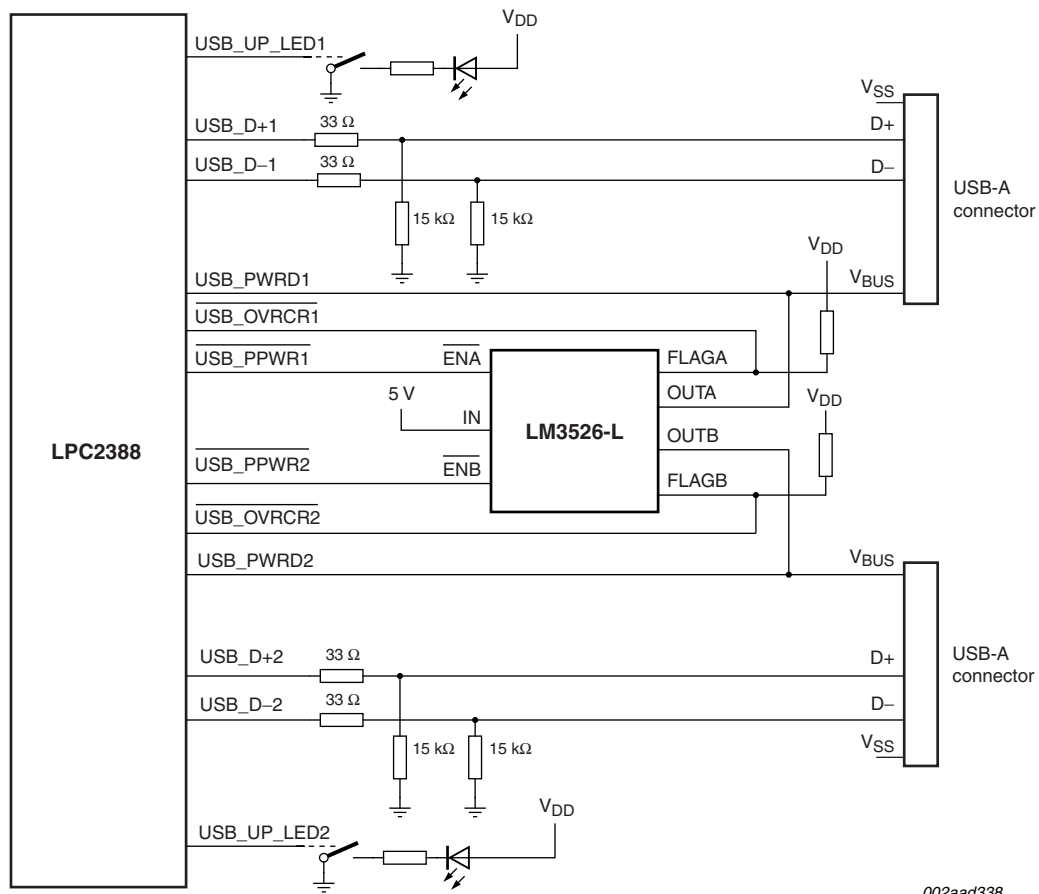
Fig 14. LPC2388 USB OTG port configuration: USB port 1 host, USB port 2 host
