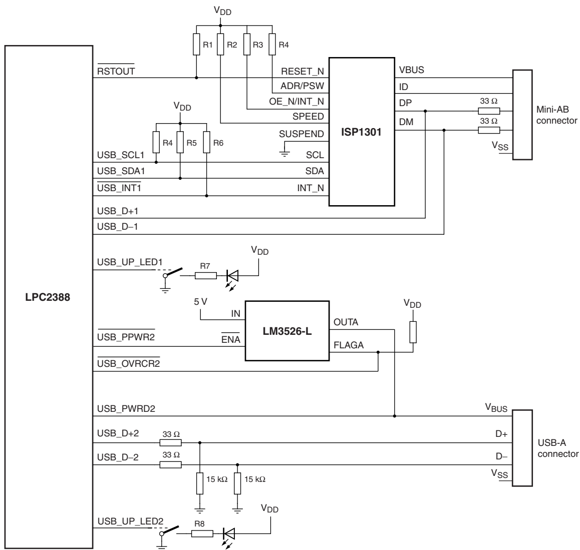
Fig 11. LPC2388 USB OTG port configuration: USB port 1 OTG dual-role device, USB port 2 host
