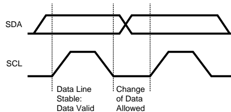
Figure 15. Bit Transfer
