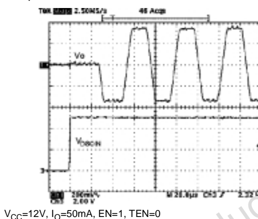
Figure 35: DSQIN Tone Enable Transient Response
