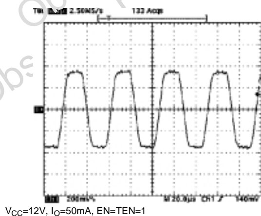
Figure 34: 22kHz Tone
