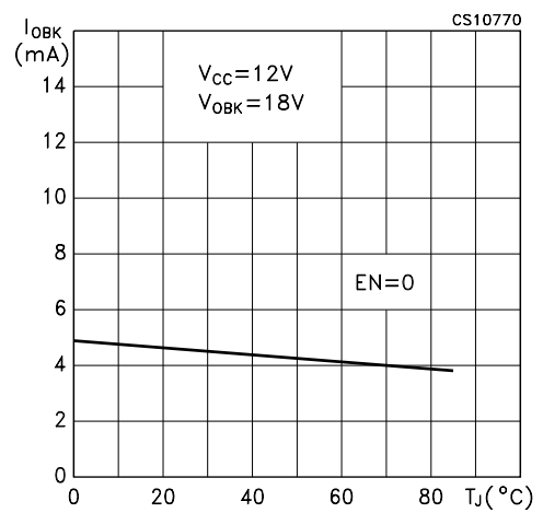
Figure 31: Output Backward Current vs Temperature
