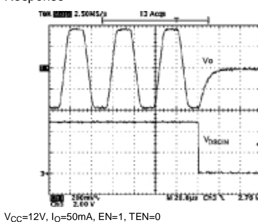
Figure 37: DSQIN Tone Disable Transient Response
