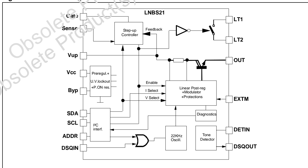
Figure 1: Schematic Diagram.
