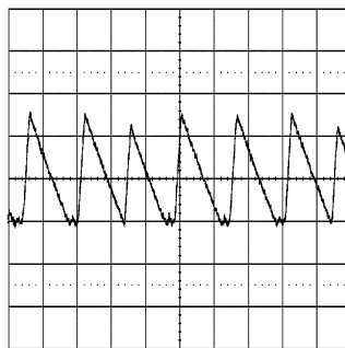
Figure 31. Transition Mode Operation V_{IN} = 24 \text{ V} , V_O = 3.3 \text{ V} , I_O = 0.35 \text{ A} 2 \mu\text{s/div}
