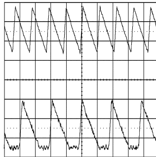
Figure 30. CCM and DCM Operating Modes V_{IN} = 24 \text{ V} , V_O = 3.3 \text{ V} , I_O = 2 \text{ A} / 0.32 \text{ A} 2 \mu\text{s/div}
