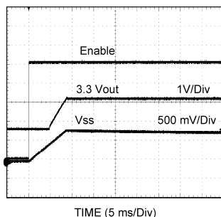
Figure 45. Prebiased Start-Up
