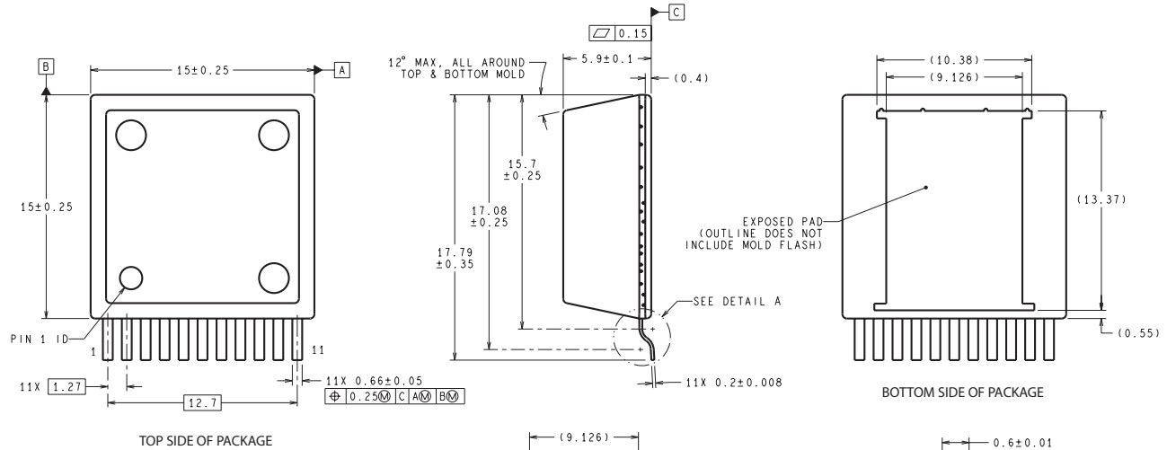
TOP SIDE OF PACKAGE
