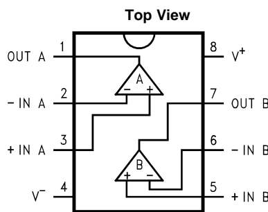
Figure 60. 8-Pin VSSOP/SOIC Package
