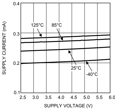
Figure 9. Supply Current vs Supply Voltage Single LMV831
