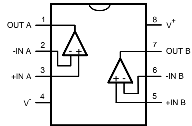
Figure 4. 8-Pin VSSOP Top View
