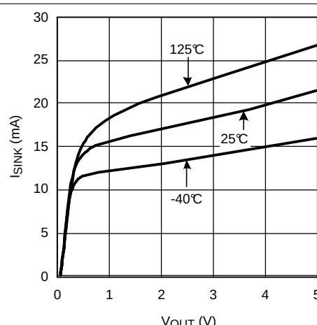
Figure 18. Sinking Current vs Output Voltage
