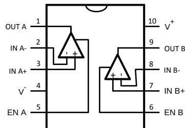
LMV792 DGS Package 10-Pin VSSOP Top View
