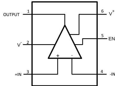
Pin Functions—LMV791
