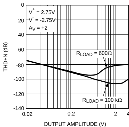
Figure 29. THD+N vs Peak-to-Pek Output Voltage ( V_{OUT} )
