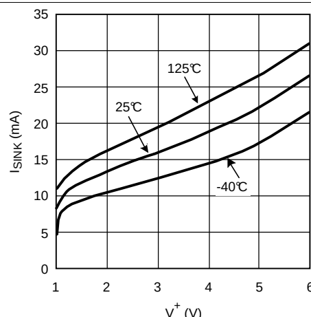
Figure 16. Sinking Current vs Supply Voltage
