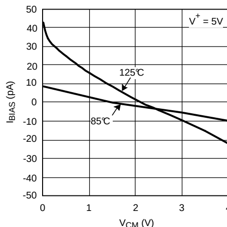
Figure 14. Input Bias Current vs V_{CM}
