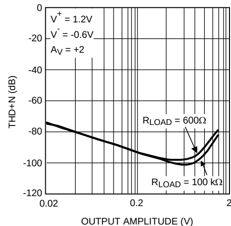
Figure 28. THD+N vs Peak-to-Pek Output Voltage ( V_{OUT} )
