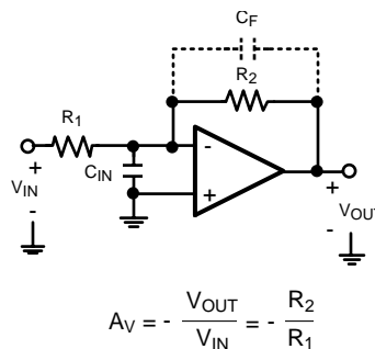
Figure 47. Inverting Amplifier
