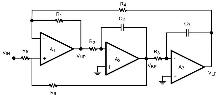
Figure 38. State Variable Active Filter
