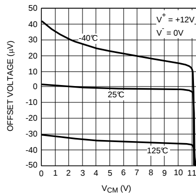
Figure 4. Offset Voltage vs V_{CM}
