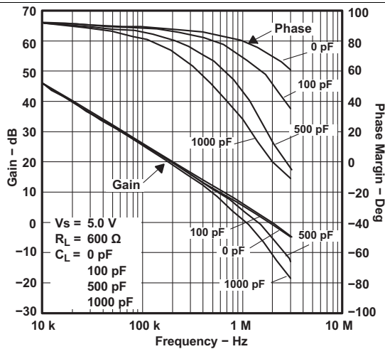
Figure 3. LMV321 Frequency Response vs Capacitive Load
