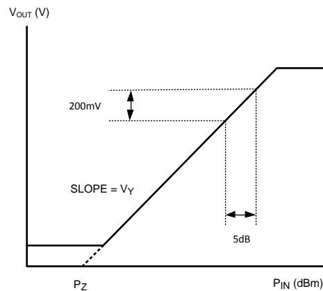
Figure 19. V_{\text{OUT}} vs. RF Input Power P_{\text{IN}}
