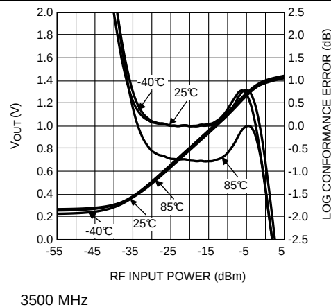
Figure 12. Mean Output Voltage and Log Conformance Error vs RF Input Power
