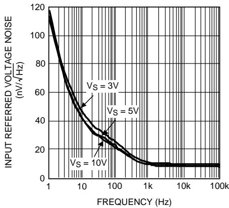
Figure 31. Input Voltage Noise vs Frequency
