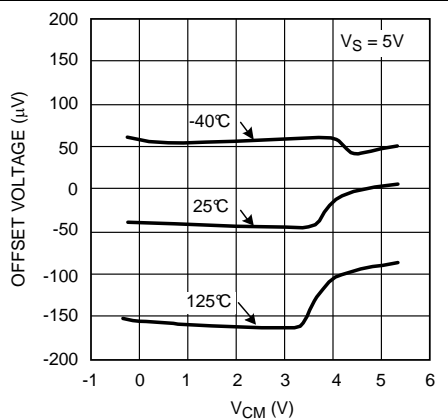
Figure 11. Offset Voltage vs V_{CM}
