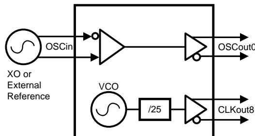
Figure 12. Start-Up Clock Using XO or Other External Reference
