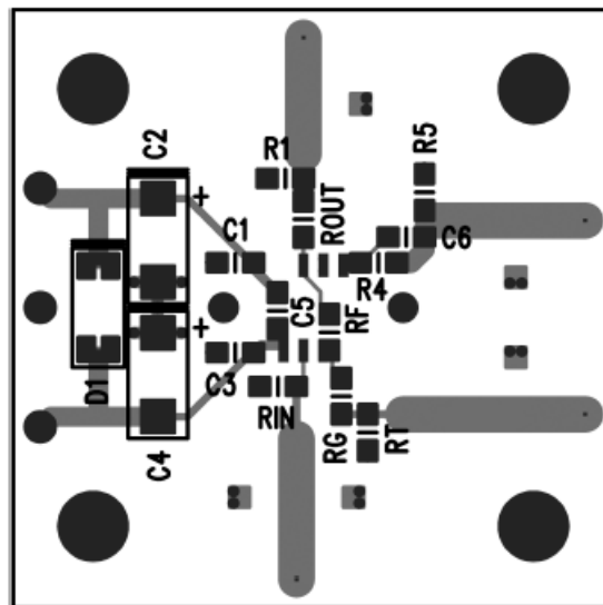
Figure 60. LMH6642/LMH6643/LMH6644 Layer 2
