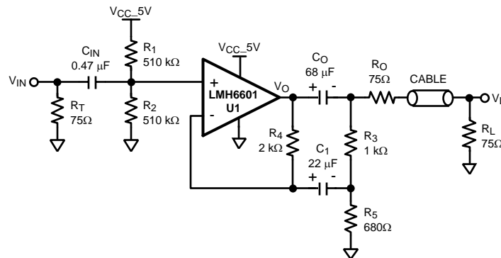
Figure 61. AC-Coupled Video Amplifier/Driver With SAG Compensation
