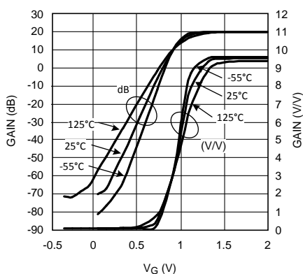
Figure 1. Gain vs. V_G
