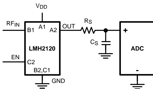
Figure 59. Low-Pass Output Filter for Residual Ripple Reduction
