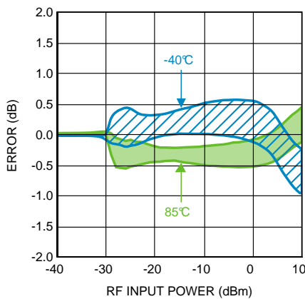
Figure 35. Temperature Variation (50 Units) vs. RF Input Power at 3500 MHz
