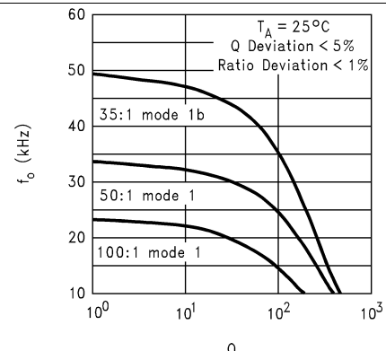
Figure 22. Maximum f_0 vs Q at V_s = \pm 7.5 \text{ V}
