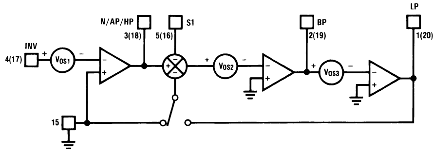
Figure 59. Offset Voltage Sources
