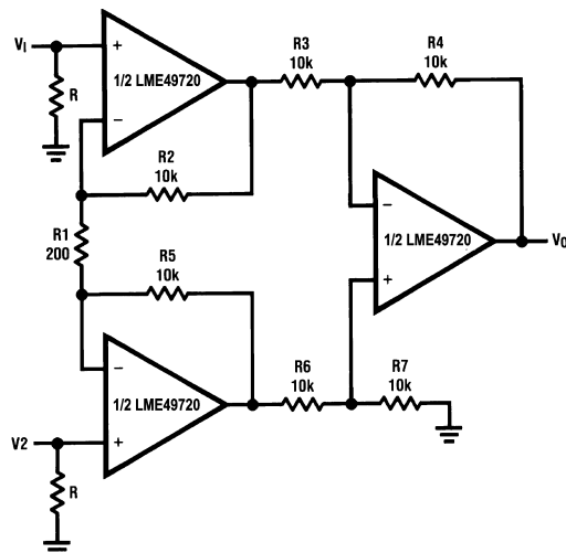
Figure 124. RIAA Preamp
