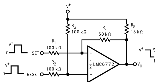
Figure 34. Bi-Stable Multivibrator
