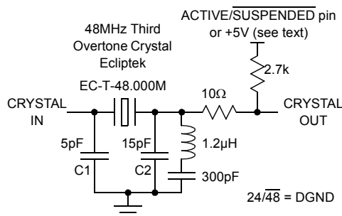
Figure 46: 48 MHz Crystal Oscillator Circuit
