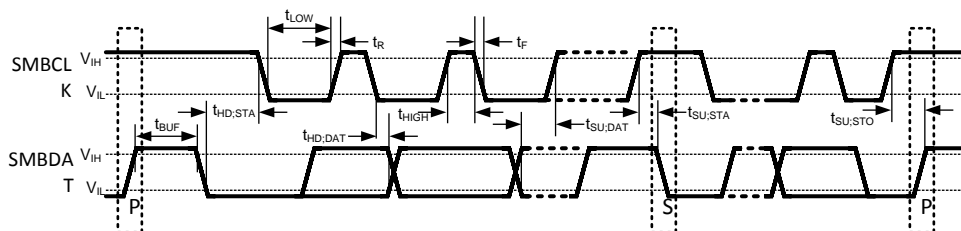
Figure 1. SMBus Communication
