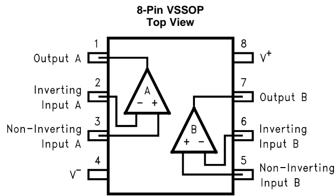
Pin Functions
