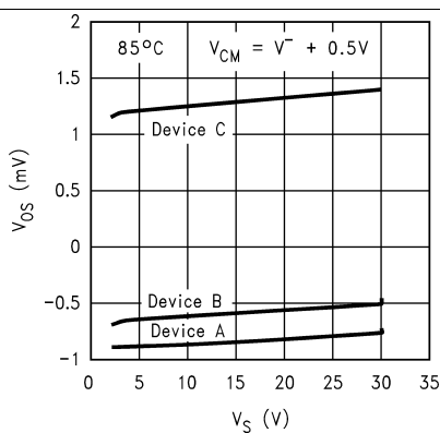
Figure 4. V_{OS} vs. V_S for 3 Representative Units
