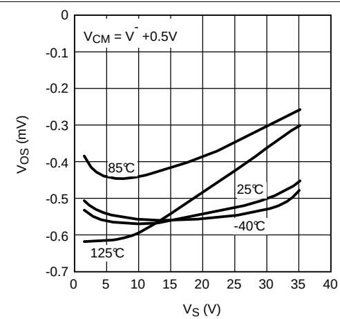
Figure 18. V_{OS} vs. V_S (Unit 2)
