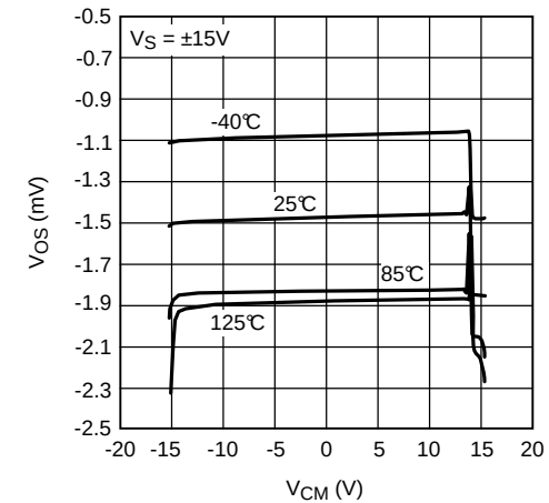
Figure 16. V_{OS} vs. V_{CM} (Unit 3)
