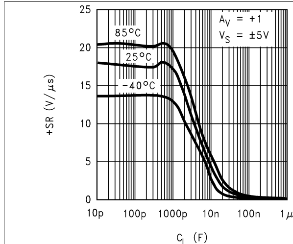
Figure 62. +SR vs. Capacitive Load
