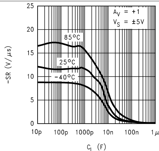
Figure 63. -SR vs. Capacitive Load
