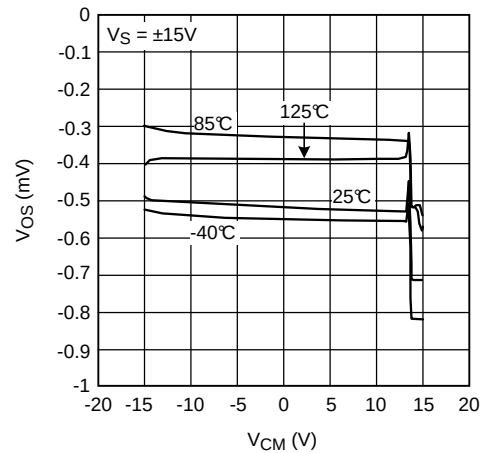
Figure 15. V_{OS} vs. V_{CM} (Unit 2)
