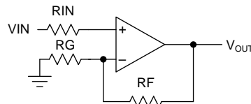
Figure 31. Schematic Representation
