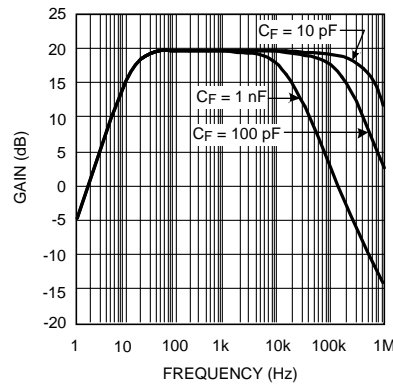
Figure 46. Frequency Response of the Non-Inverting Preamp
