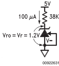
FIGURE 3. 1.2V Reference
