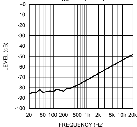
Figure 9. Input Floating
