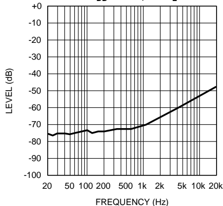
Figure 13. Input Floating
