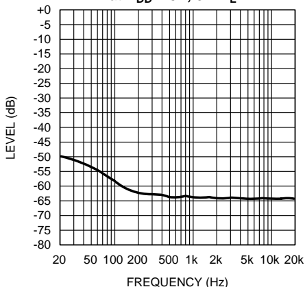
Figure 8. Input terminated with 10\Omega
