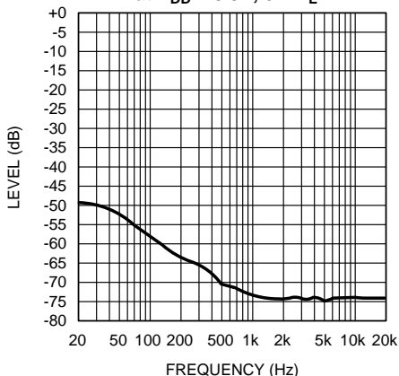
Figure 10. Input Floating
