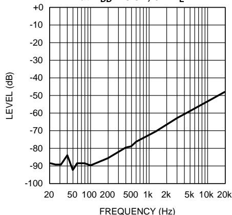
Figure 11. Input Floating
