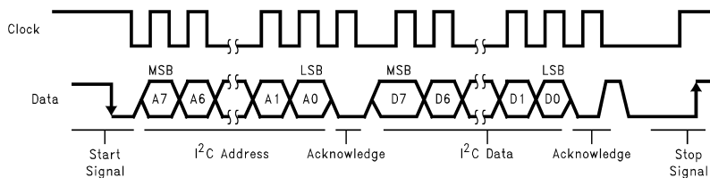
Figure 14. I 2 C Bus Format
