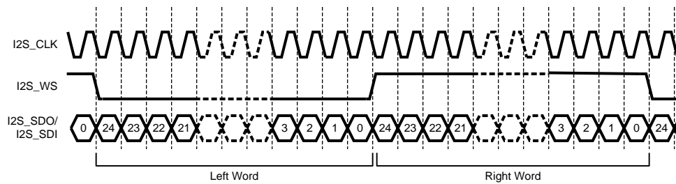
Figure 20. I 2 S Serial Data Format (Left Justified)
