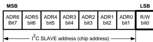
Figure 5. I 2 C Chip Address
